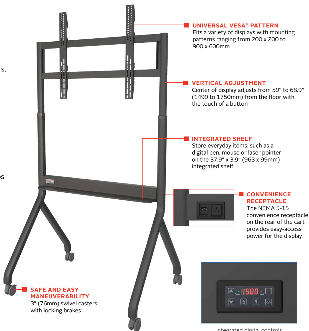
Integrated digital controls at the rear of the cart
