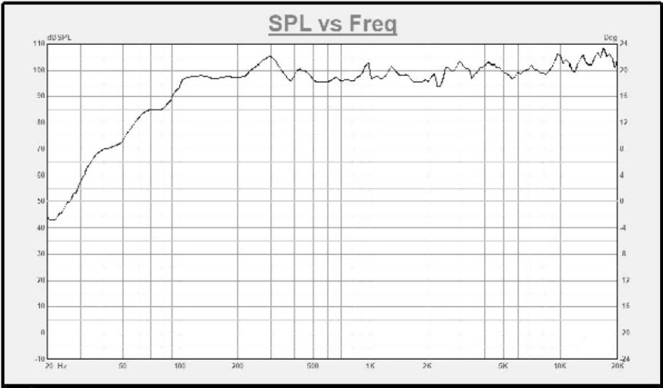
Response curve (SPL/Impedance vs. Frequency)
