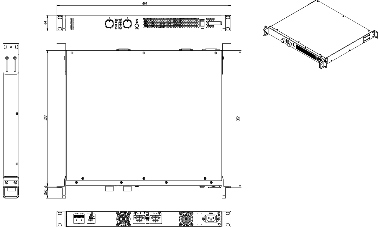
Ecler AURA-2B900 Mechanical Diagram
