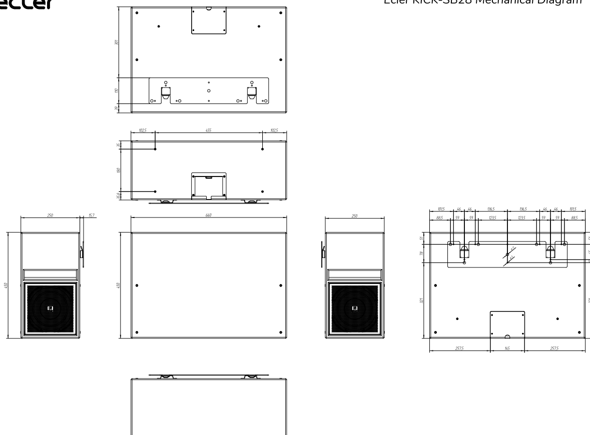
Ecler KICK-SB28 Mechanical Diagram
